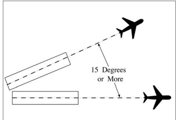
FIG 5-8-4 Nonintersecting Runway Departures
