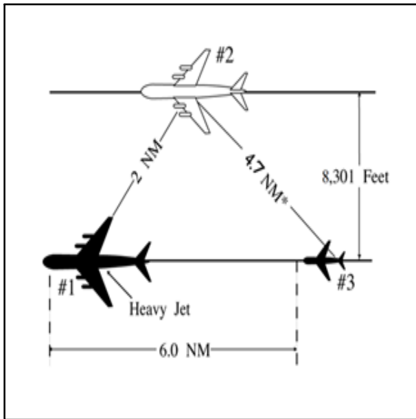
FIG 5-9-5 Simultaneous Dependent Approaches
